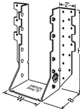
FIGURE 9—HHUS SERIES HANGER (See Table 9)
