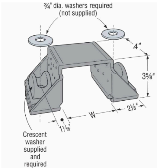
HGT-2 Heavy Girder Tiedown (HGT-3 and HGT-4 similar)
